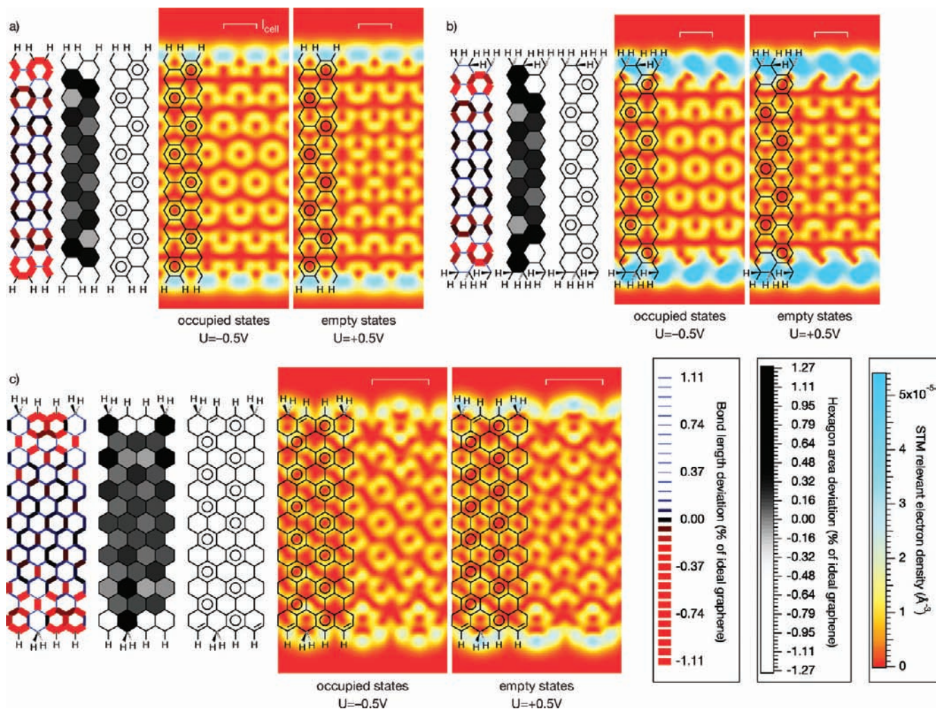
Figure 6. Graphene ribbons with one unique Clar formula, class 1CF: (a) ac(11) ribbon with width index w = 22 ; (b) ac(22) ribbon with width index w = 21 ; (c) zz(211)-interlock ribbon with w = 13 . Subfigures show (from left to right) bond lengths, hexagon areas, Clar formulas, negative bias STM images, and positive bias STM images. The scales of the bond lengths and hexagon areas show the deviations from the values of ideal graphene, 1.427 Å and 5.293 Å 2 , respectively, in percent. All scales are valid throughout this section.
